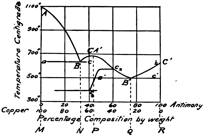
Fig. 51. Freezing-point Curve of Copper-antimony Alloys.
